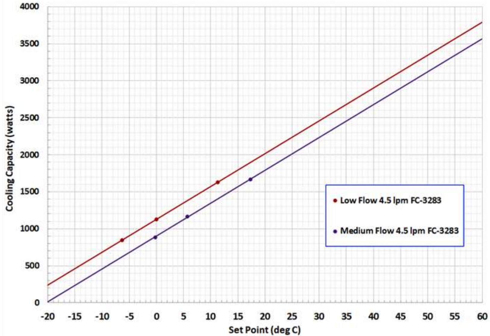
Low / Medium Flow ThermoRack 1801 Cooling Curves 20°C PCW
